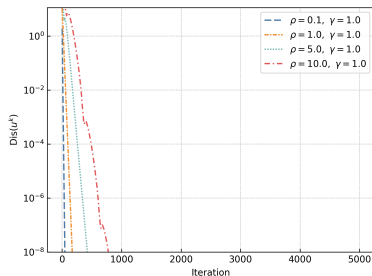
(b) \rho = \{0.1, 1.0, 5.0, 10.0\}, \gamma = 1.0
