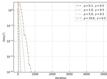
(a) \rho = \{0.1, 1.0, 5.0, 10.0\}, \gamma = 0.5
